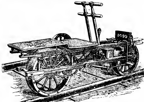
Fig. 5605. SHEFFIELD ODOMETER VELOCIPEDE-CAR. For measuring track.
